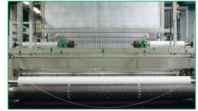
Figure 11 Secugrid® production
