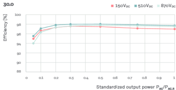
Fronius Verto 30.0
